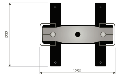
Instron® 8803 Dimensions (All Dimensions are in mm)
